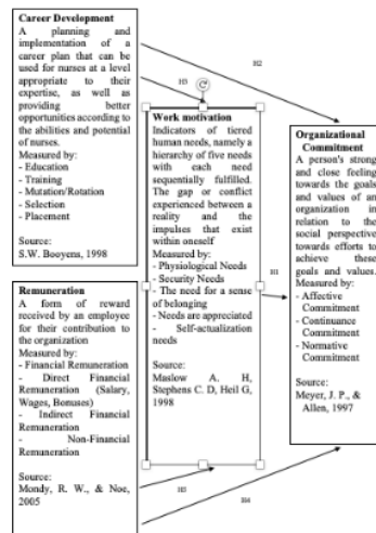
Figure 1 Theoretical Framework
