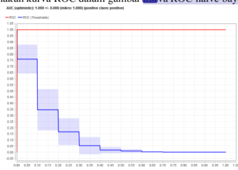
Gambar 2. Kurva ROC Naive Bayes
