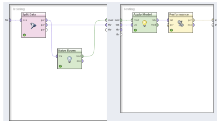
Gambar 1. Model Pengujian Validasi Naive Bayes
